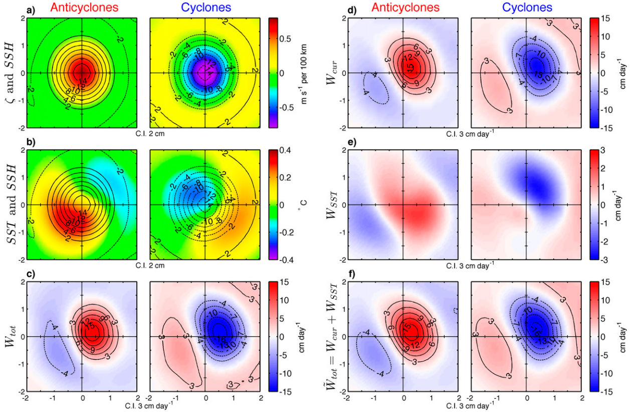
FIG. 14. As in Fig. 13, but for SIO ( 20^{\circ} – 35^{\circ}\text{S} , 80^{\circ} – 115^{\circ}\text{E} ).
